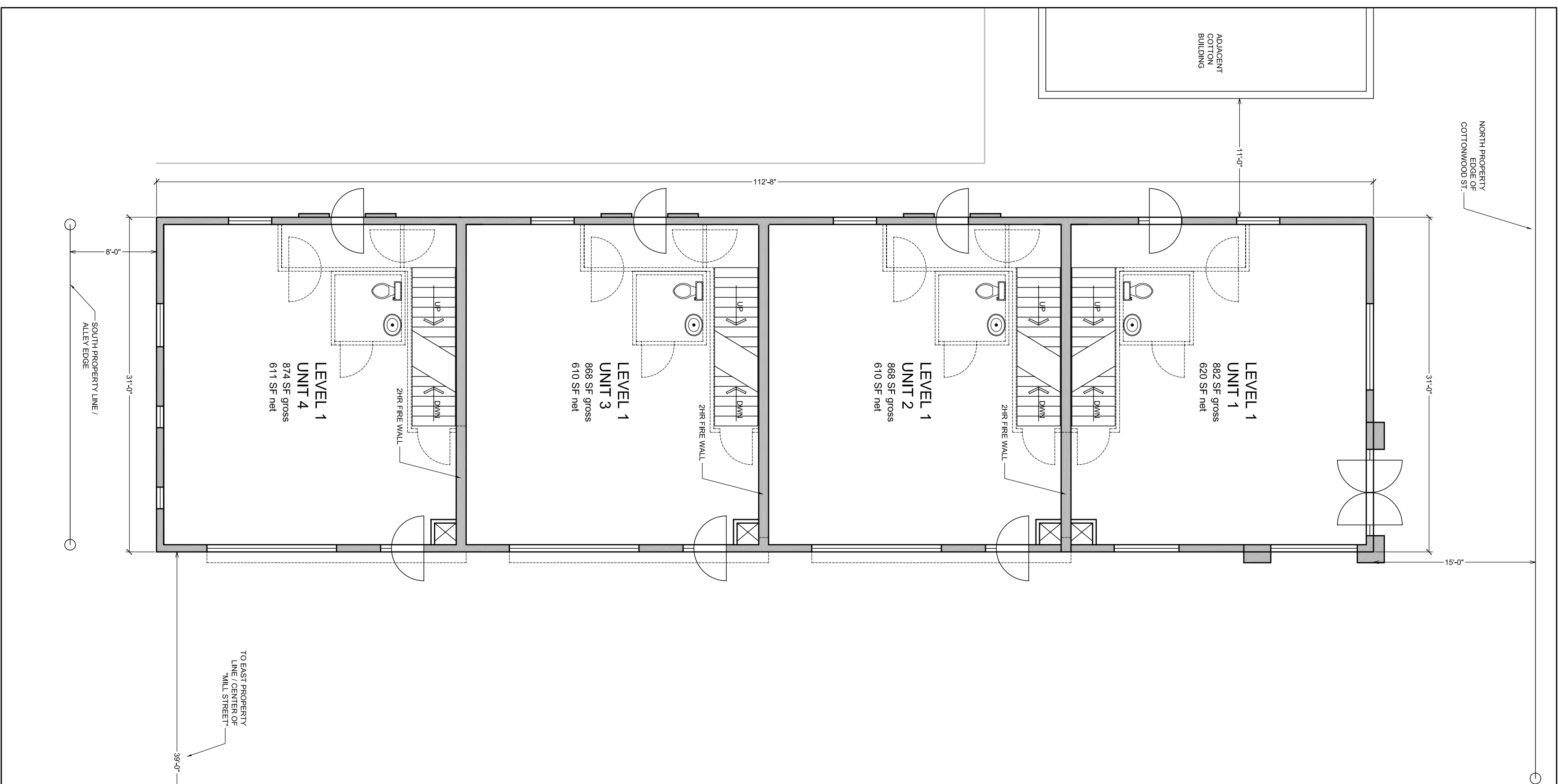
LEVEL 1 FLOOR PLAN SCALE: 1/8" = 1'
