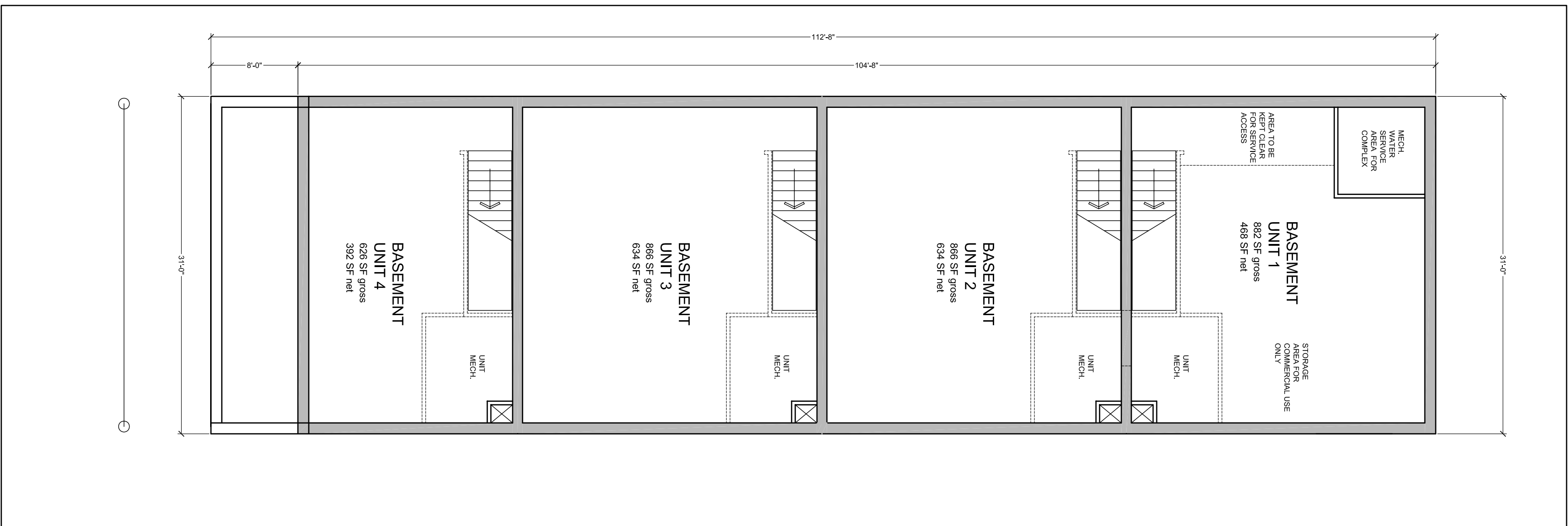
BASEMENT LEVEL FLOOR PLAN SCALE: 1/8" = 1'
